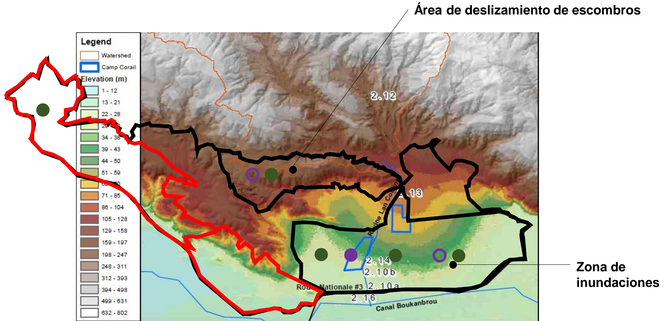
Figure 2.11 – Topographical map of the study area based on adjusted elevation values from TanDEM-X. The location of photos in this chapter is marked by their number
